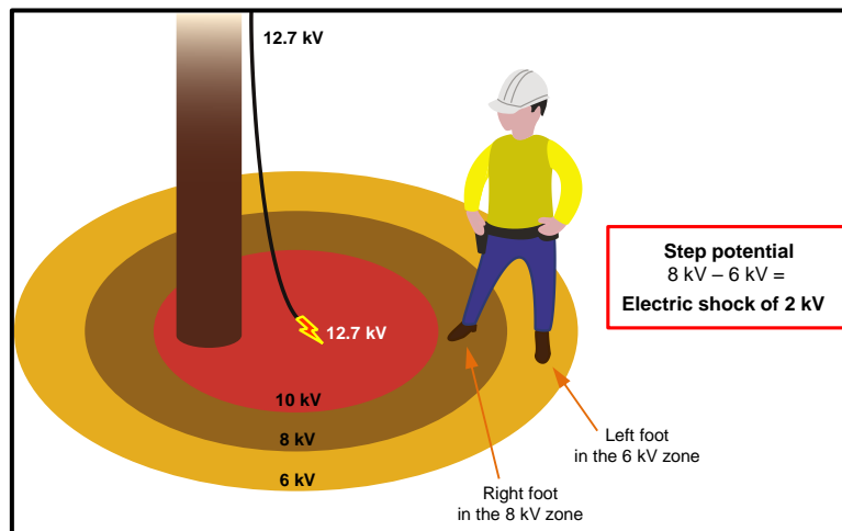
Figure 2 - Step potential
