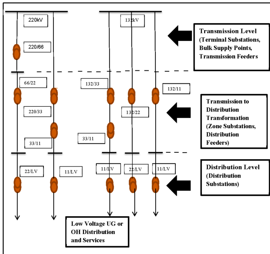
Figure 5 – Functional Components of a Distribution System
