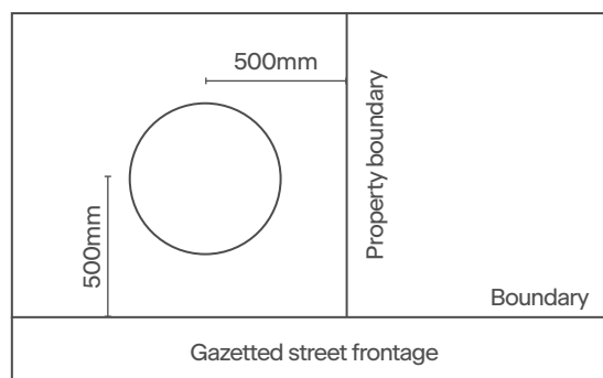
Mandatory location of pillar
